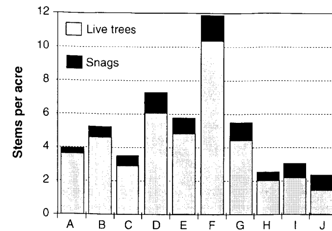
Figure 11 —Density of standing live trees (light shading) and standing snags (dark shading) in d.b.h. classes 21 inches or greater, classified by habitat type groups. A=warm, dry; B=moderately warm, dry; C=moderately cool, dry; D=warm, moist; E=cool, moist; F=wet; G=moderately cool, moist; H=cool, moderately dry; I=cool, moderately dry, J=cold.
