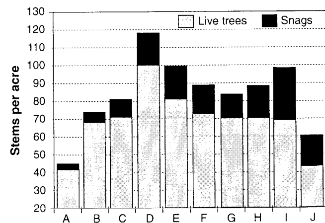
Figure 10 —Density of standing live trees (light shading) and standing snags (dark shading) in d.b.h. classes 9 inches or greater, classified by habitat type groups. A = warm, dry; B = moderately warm, dry; C = moderately cool, dry; D = warm, moist; E = cool, moist; F = wet; G = moderately cool, moist; H = cool, moderately dry; I = cool, moderately dry, J = cold.
