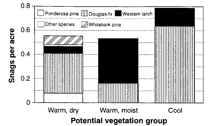
Figure 7 —Snag (d.b.h. 21 inches or greater) density on uncut plots within FIA-designated Douglas-fir cover types by the three most common potential vegetation groups, showing the proportion made up by ponderosa pine, Douglas-fir, western larch, whitebark pine, and all other species.
