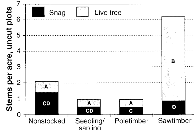
Figure 3 —Standing stems per acre (21 inches or greater) in uncut plots, by the four successional stages identified by the FIA program, showing both snags (dark shading) and live trees (light shading). Bars with the same letter are not significantly different at P < 0.05 (Tukey's Honestly Significant Difference Post-Hoc Test).
