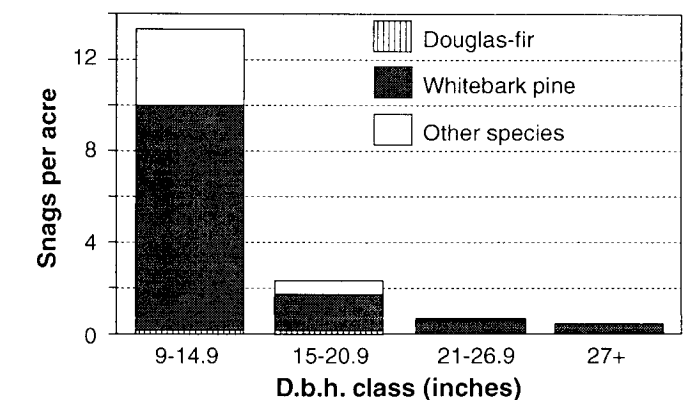
Figure 13 —Snag density in the cold habitat type group by d.b.h. class, showing the predominance of whitebark pine snags.
