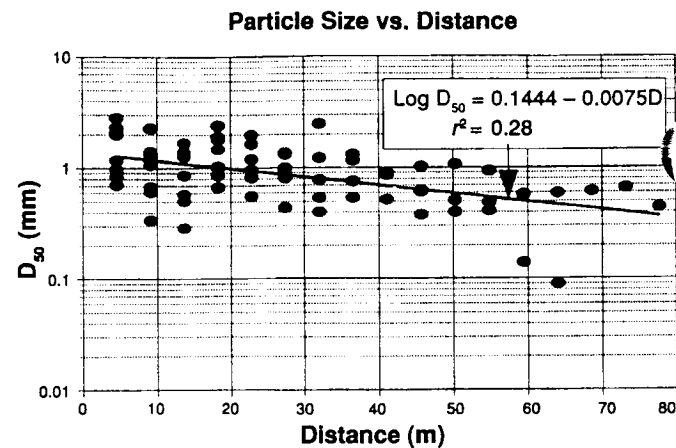
Figure 7—Median sediment particle size ( D_{50} ) as a function of travel distance.
