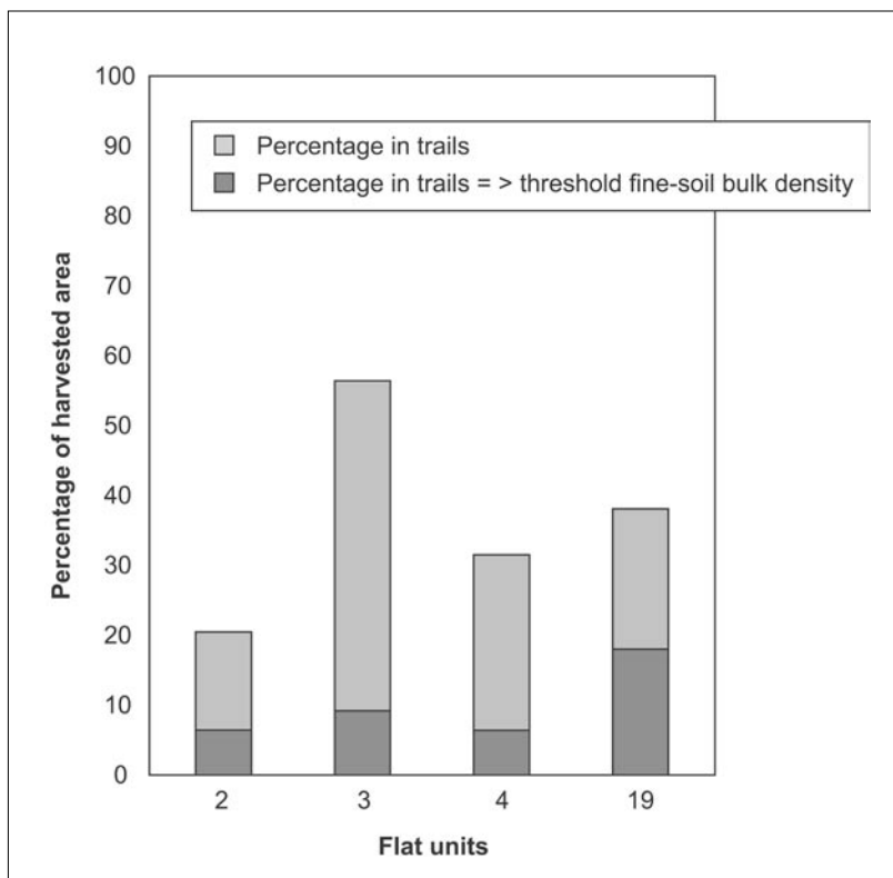
Figure 8—Percentage of harvested area in trails, and area in trails with fine-soil bulk density 20 percent greater than before-harvest mean bulk density, flat terrain.
