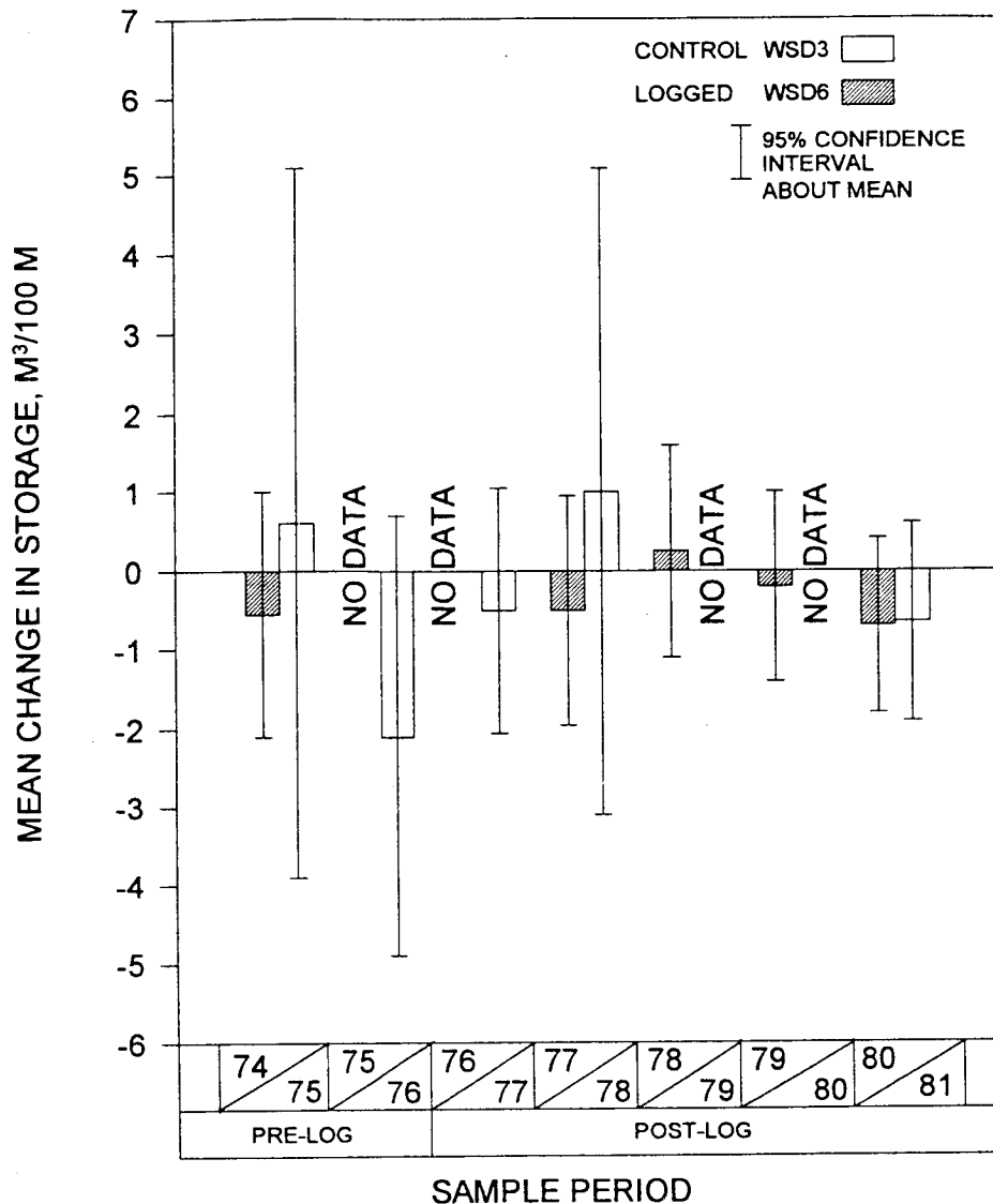
FIGURE 6. Pre- and postdisturbance net changes between years in channel bottom lithic sediment volumes on WSD3 (control) and WSD6 (logged and burned).
