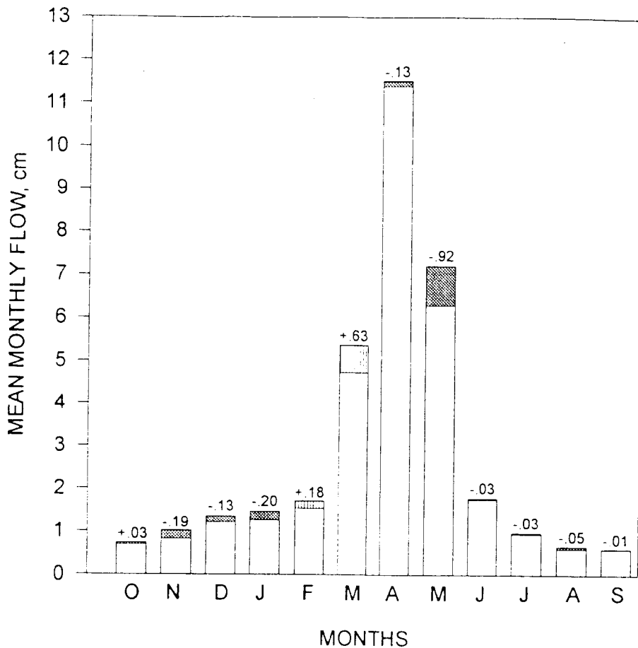
FIGURE 3. Summary of regression analyses of monthly flows before and after disturbance. Shaded areas at the top of each bar represent the difference between the measured and the predicted monthly water yield on WSD6 (logged and burned). Type of shading and numbers indicate the direction and magnitude (cm) of change.
