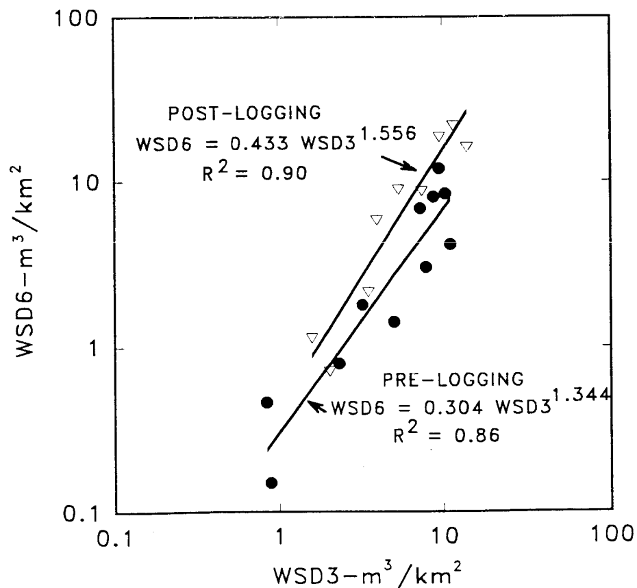
FIGURE 4. Pre- and postdisturbance regression analyses of annual sediment yield as measured in the sediment basins for WSD6 (logged and burned) vs. WSD3 (control).
