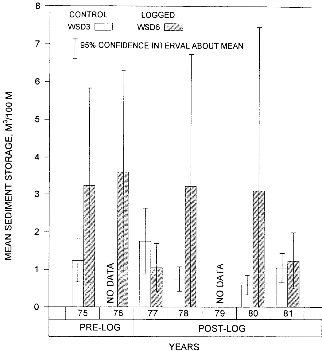
FIGURE 5. Pre- and postdisturbance average channel sediment storage behind obstructions on WSD3 (control) and WSD6 (logged and burned).
