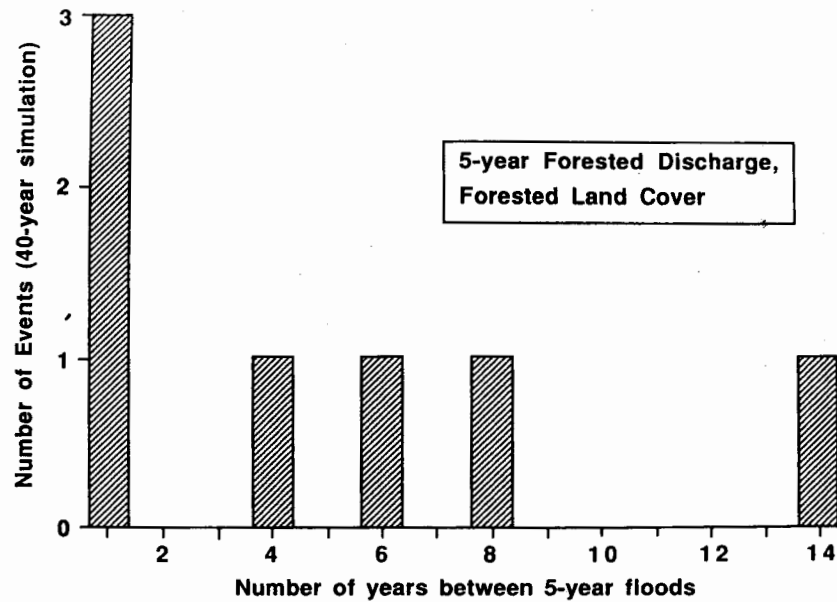
Fig. 5. HSPF simulation of the Hylebos Creek basin in southwest King County, Washington, under fully forested land cover. Bars show the number of years separating discharge events of 5-year recurrence or greater. The average separation is 5 years (40 years of simulation, 8 events), but the actual spacing varies from one year (i.e., successive years) to 14 years.
