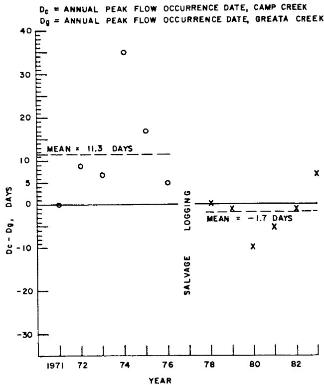
Fig. 6. The differences in annual peak flow occurrence dates, between Camp Creek and Greata Creek before (1971-1976) and after (1978-1983) the clear-cut logging in Camp Creek watershed.
